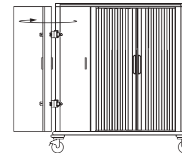
270° Pull-out door
